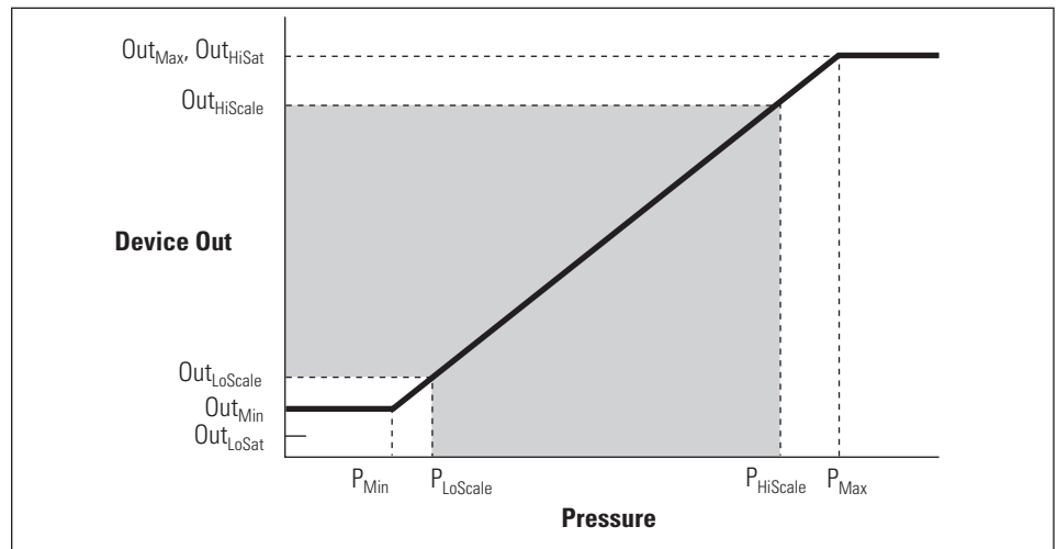
Figure 1. Typical Device Output vs. Pressure
